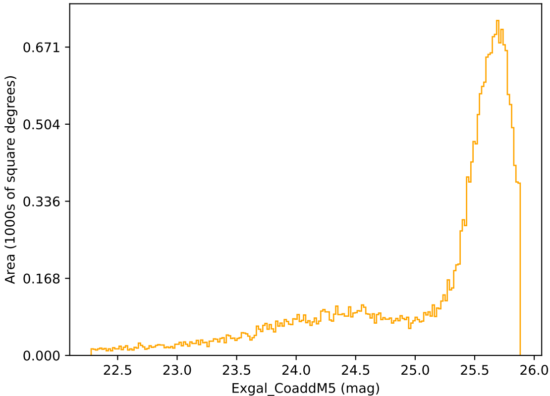
weather_cloudso30v3.4_10yrs Yr 1 r band: Exgal_CoaddM5
