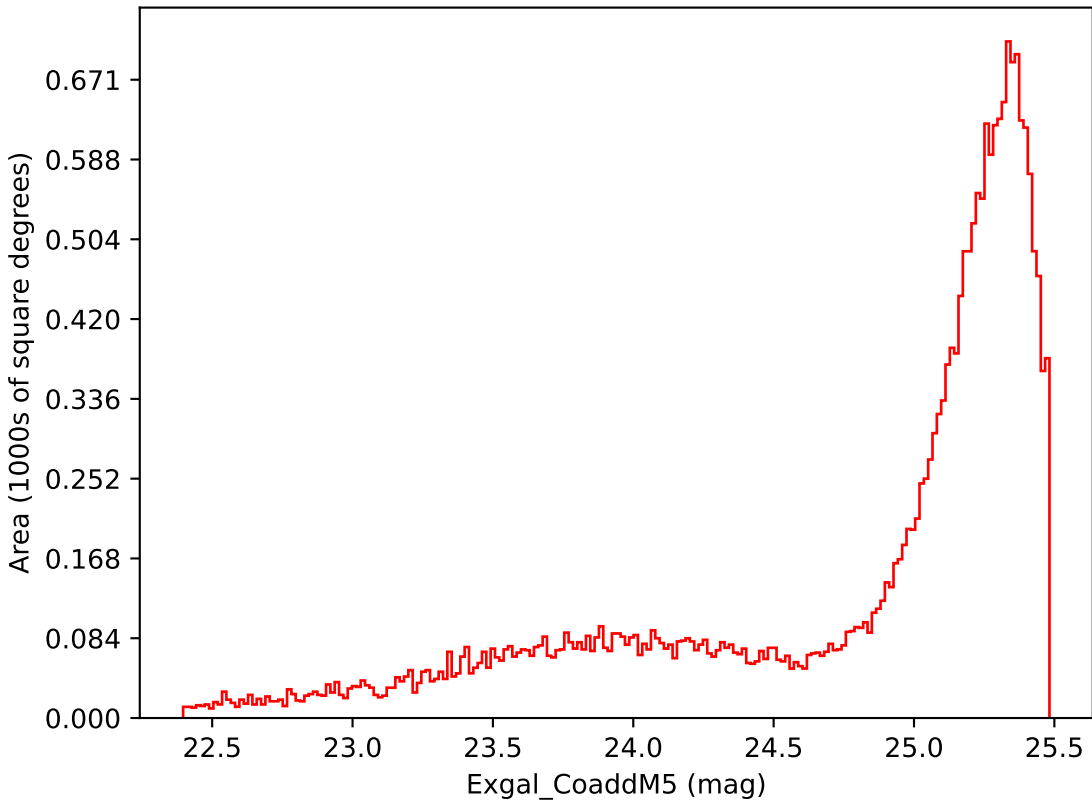
weather_cloudso30v3.4_10yrs Yr 1 i band: Exgal_CoaddM5
