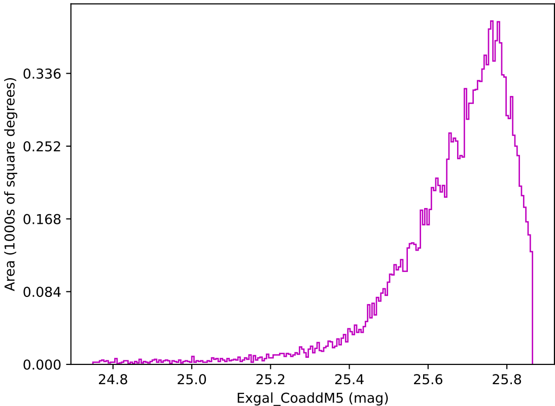
weather_cloudso30v3.4_10yrs WFD z band: Exgal_CoaddM5
