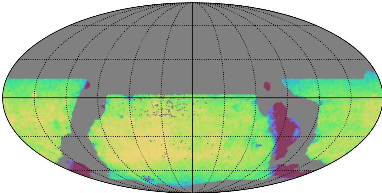
weather_cloudso30v3.4_10yrs WFD y band: Exgal_CoaddM5
