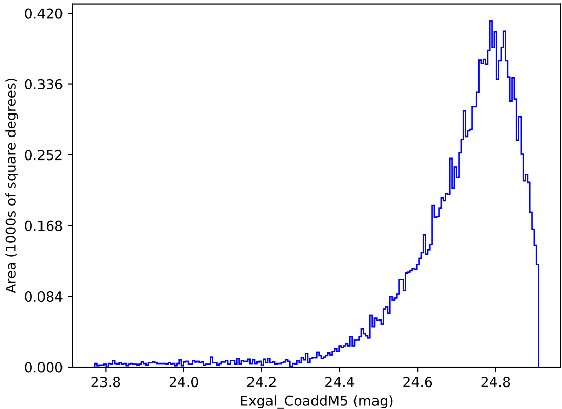
weather_cloudso30v3.4_10yrs WFD y band: Exgal_CoaddM5
