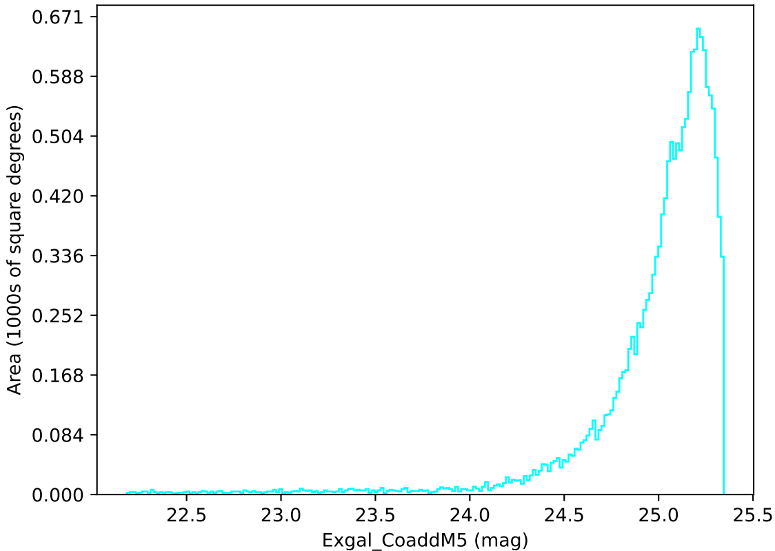
weather_cloudso30v3.4_10yrs WFD u band: Exgal_CoaddM5
