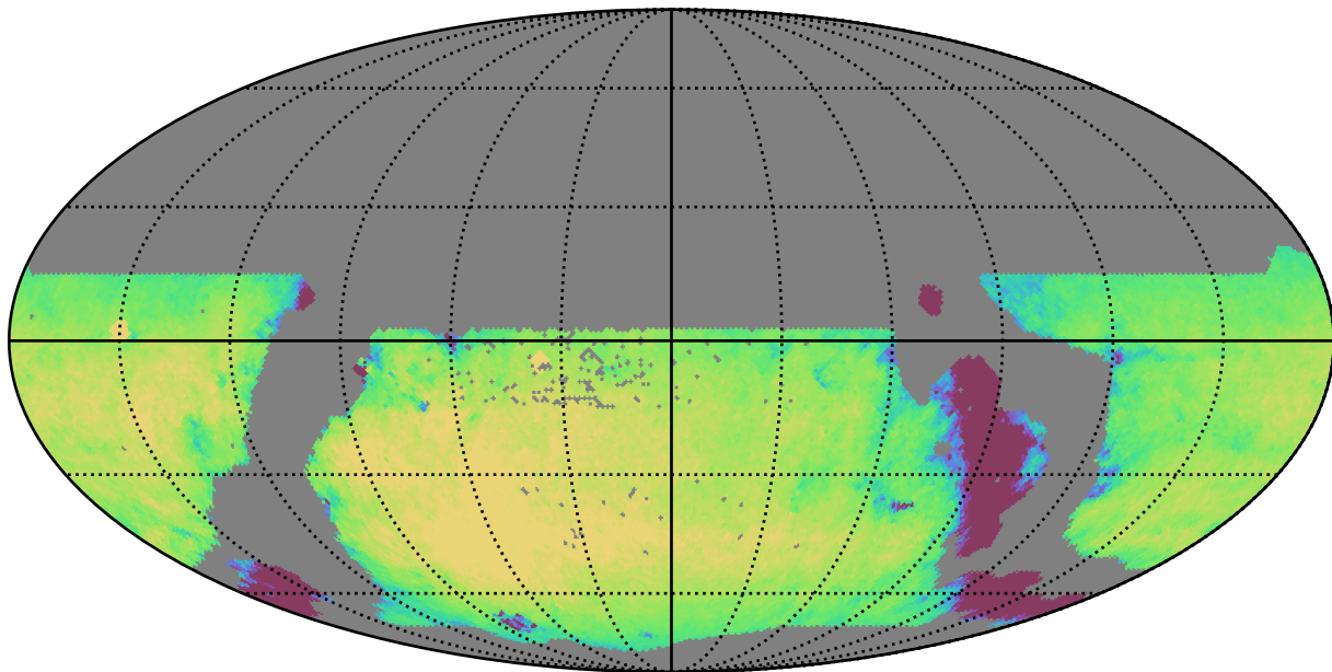
weather_cloudso30v3.4_10yrs WFD r band: Exgal_CoaddM5
