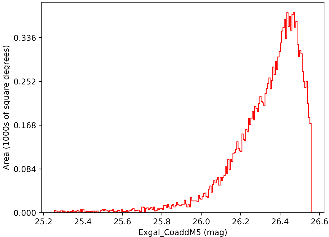
weather_cloudso30v3.4_10yrs WFD i band: Exgal_CoaddM5
