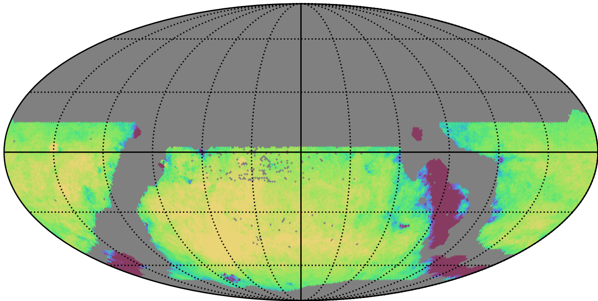
weather_cloudso30v3.4_10yrs WFD g band: Exgal_CoaddM5
