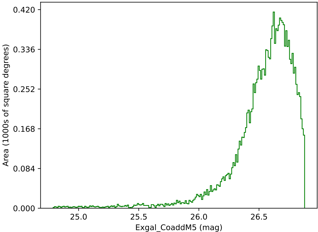
weather_cloudso30v3.4_10yrs WFD g band: Exgal_CoaddM5
