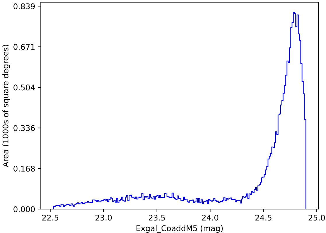
weather_cloudso30v3.4_10yrs All sky y band: Exgal_CoaddM5
