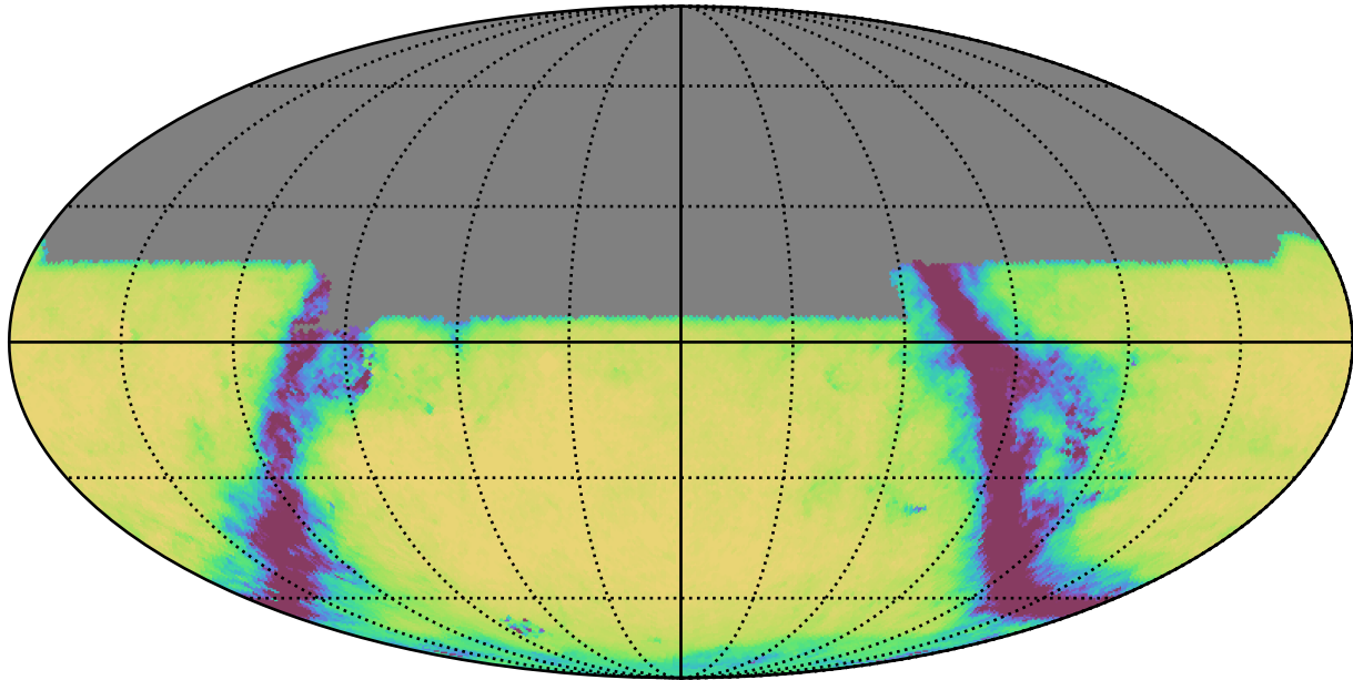
weather_cloudso30v3.4_10yrs All sky u band: Exgal_CoaddM5
