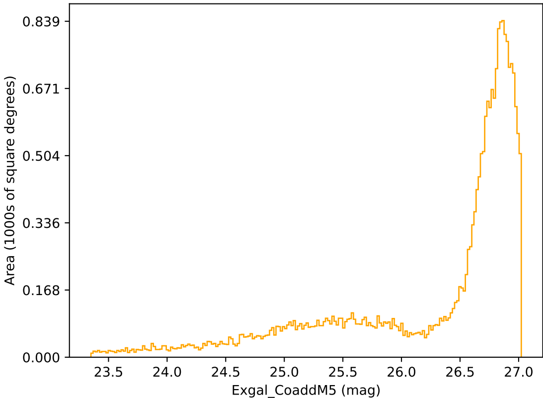
weather_cloudso30v3.4_10yrs All sky r band: Exgal_CoaddM5
