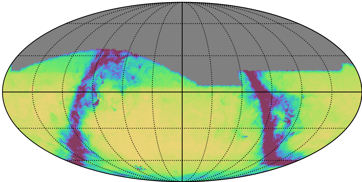
weather_cloudso30v3.4_10yrs All sky g band: Exgal_CoaddM5
