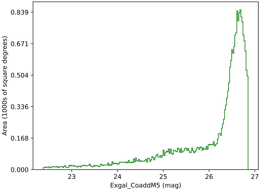
weather_cloudso30v3.4_10yrs All sky g band: Exgal_CoaddM5
