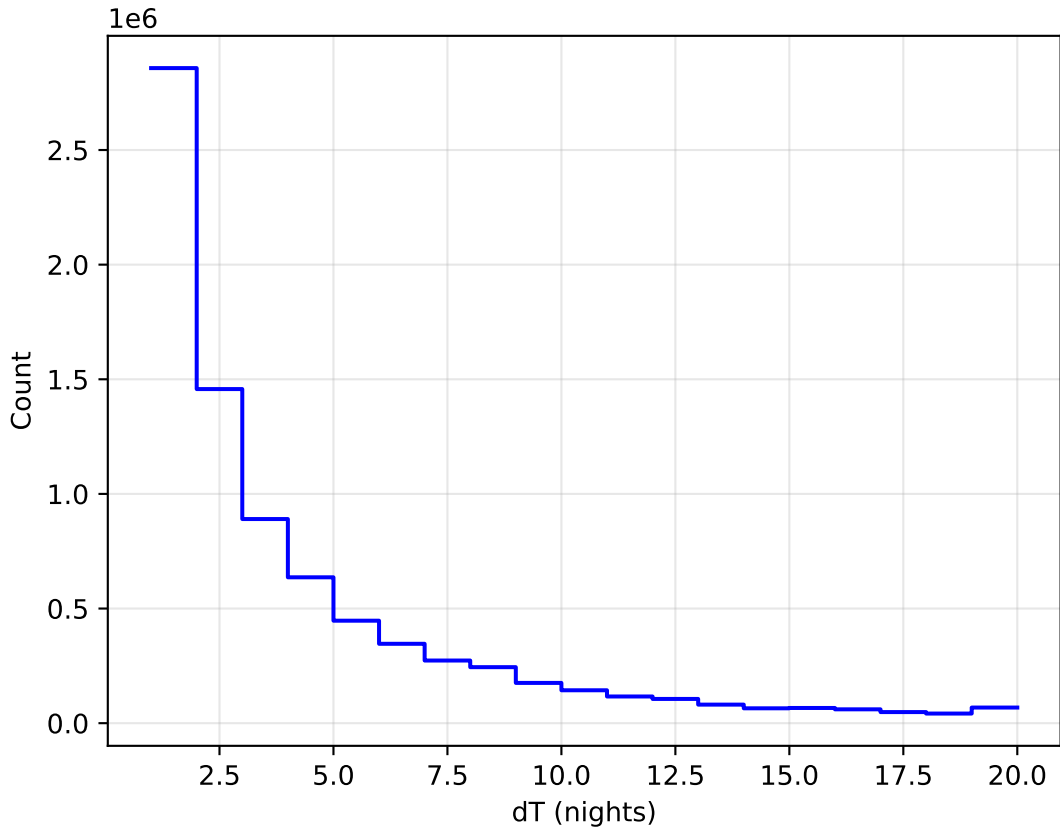
weather_cloudso30v3.4_10yrs WFD all bands: DeltaNight Histogram
