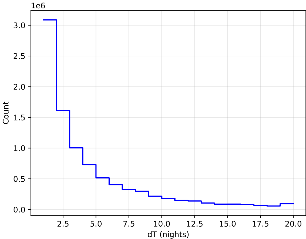
weather_cloudso30v3.4_10yrs All sky all bands: DeltaNight Histogram
