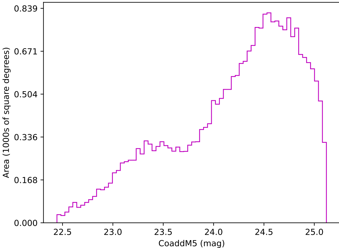
weather_cloudso30v3.4_10yrs Yr 3-4 z band: CoaddM5
