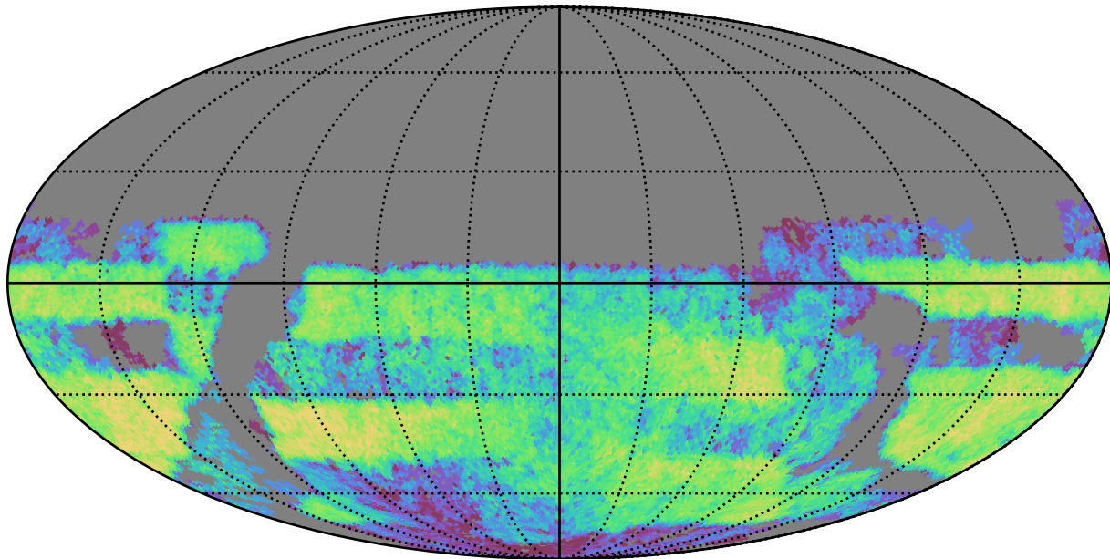
weather_cloudso30v3.4_10yrs Yr 3-4 u band: CoaddM5
