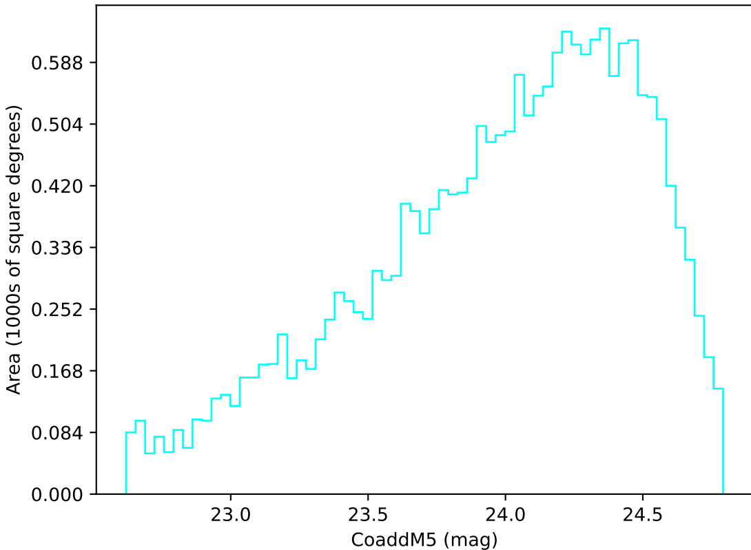
weather_cloudso30v3.4_10yrs Yr 3-4 u band: CoaddM5
