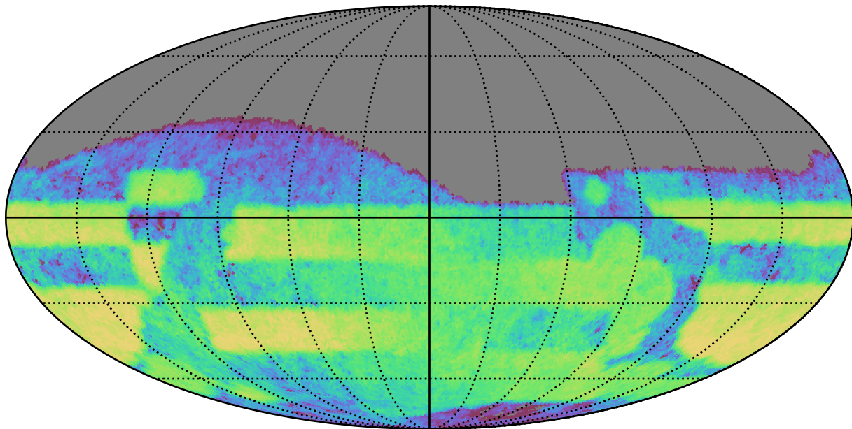
weather_cloudso30v3.4_10yrs Yr 3-4 r band: CoaddM5
