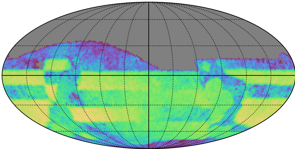
weather_cloudso30v3.4_10yrs Yr 3-4 i band: CoaddM5
