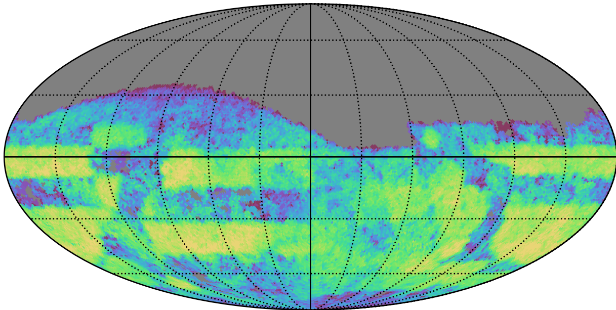
weather_cloudso30v3.4_10yrs Yr 3-4 g band: CoaddM5
