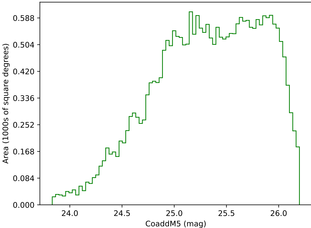
weather_cloudso30v3.4_10yrs Yr 3-4 g band: CoaddM5
