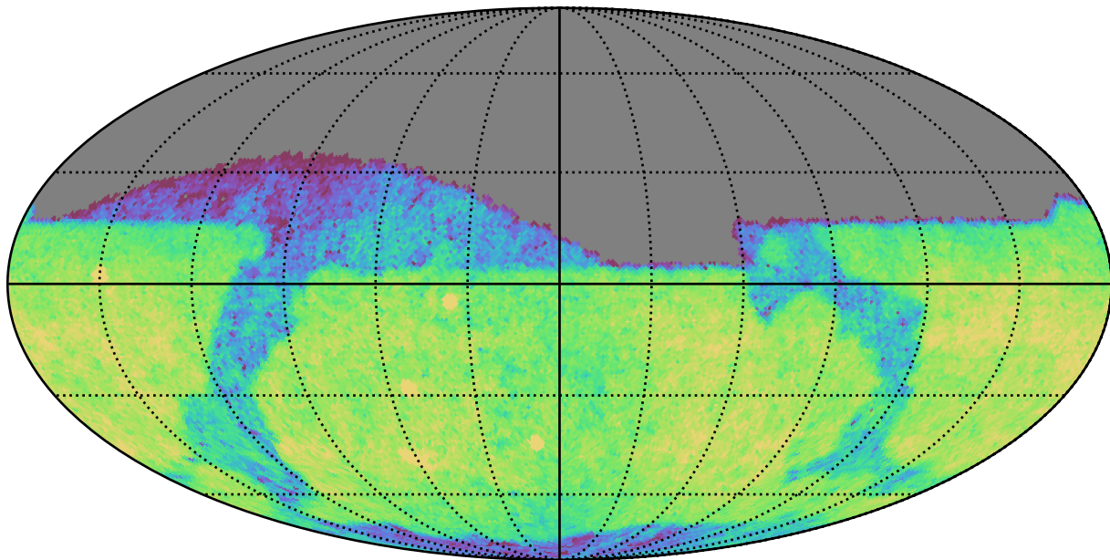
weather_cloudso30v3.4_10yrs Yr 1 z band: CoaddM5
