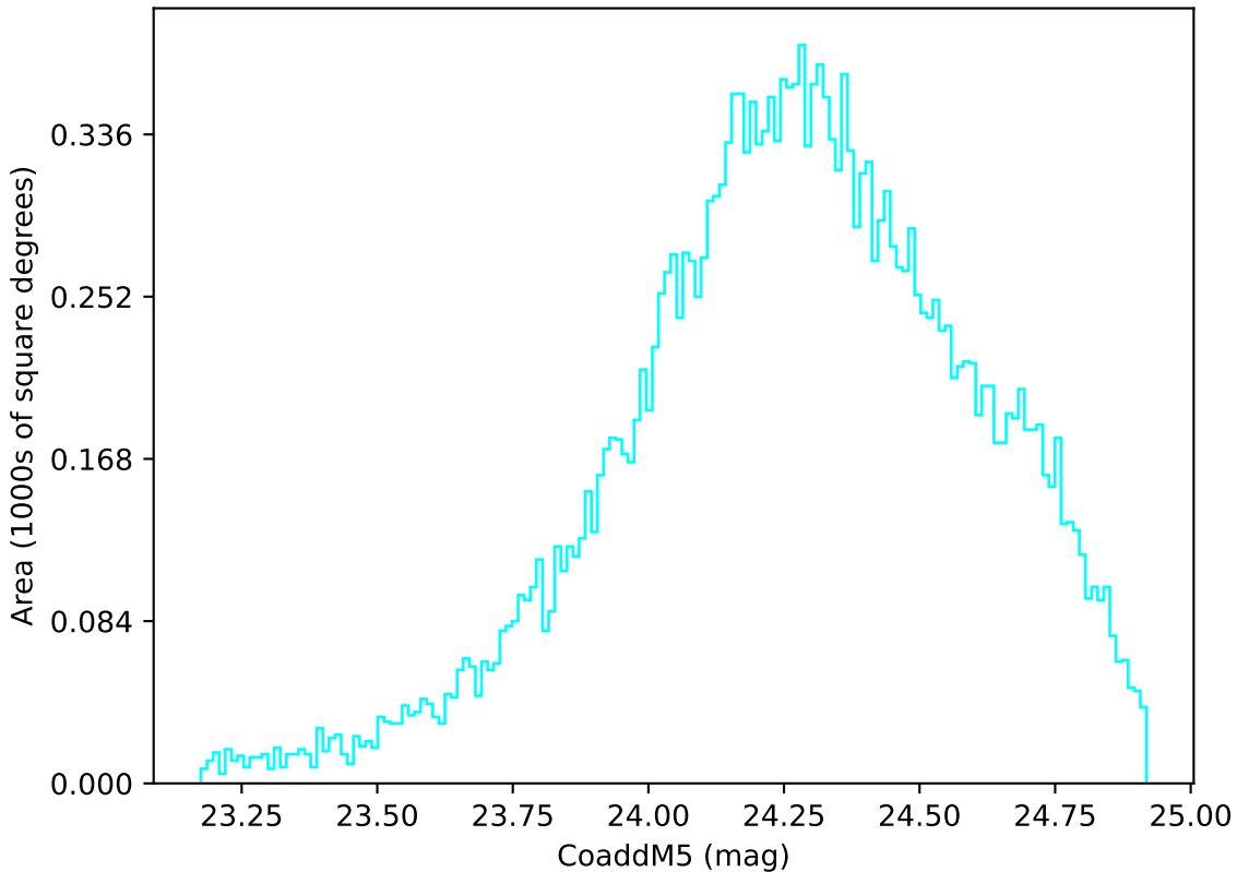
weather_cloudso30v3.4_10yrs Yr 1 u band: CoaddM5
