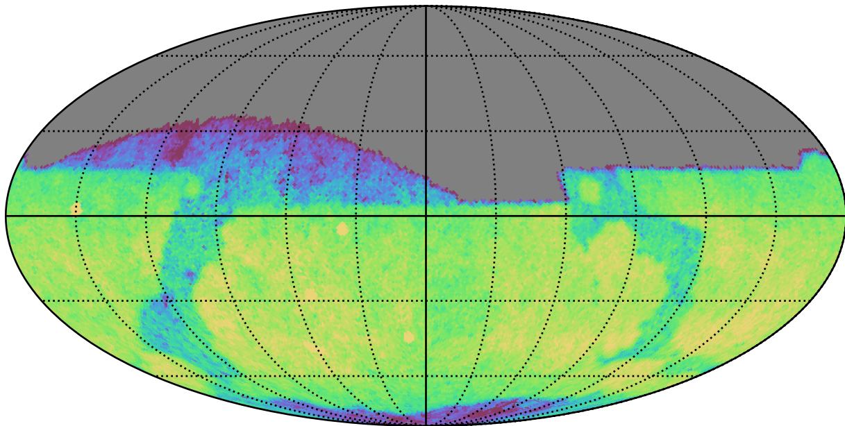
weather_cloudso30v3.4_10yrs Yr 1 r band: CoaddM5
