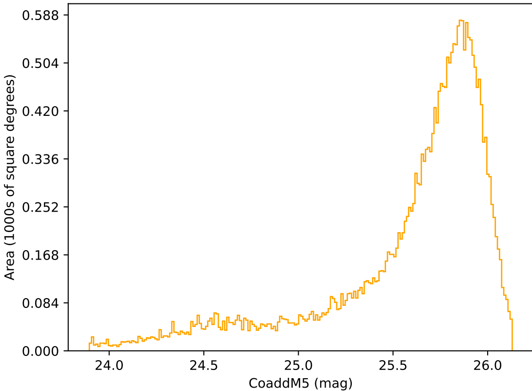
weather_cloudso30v3.4_10yrs Yr 1 r band: CoaddM5
