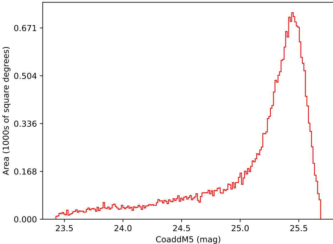
weather_cloudso30v3.4_10yrs Yr 1 i band: CoaddM5
