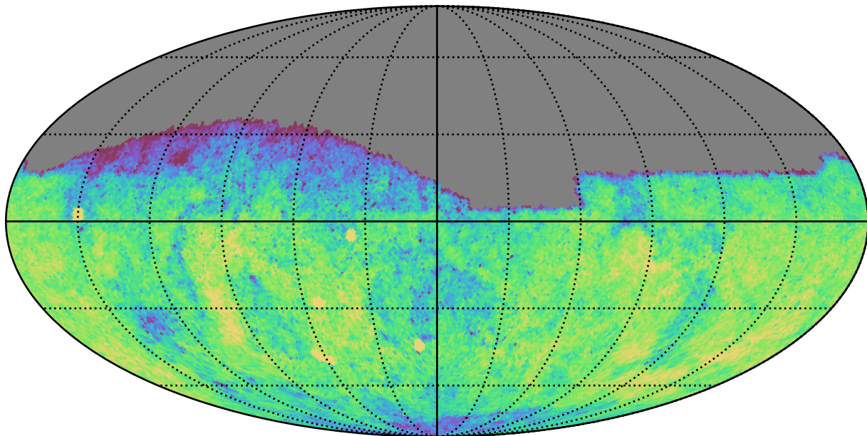
weather_cloudso30v3.4_10yrs Yr 1 g band: CoaddM5
