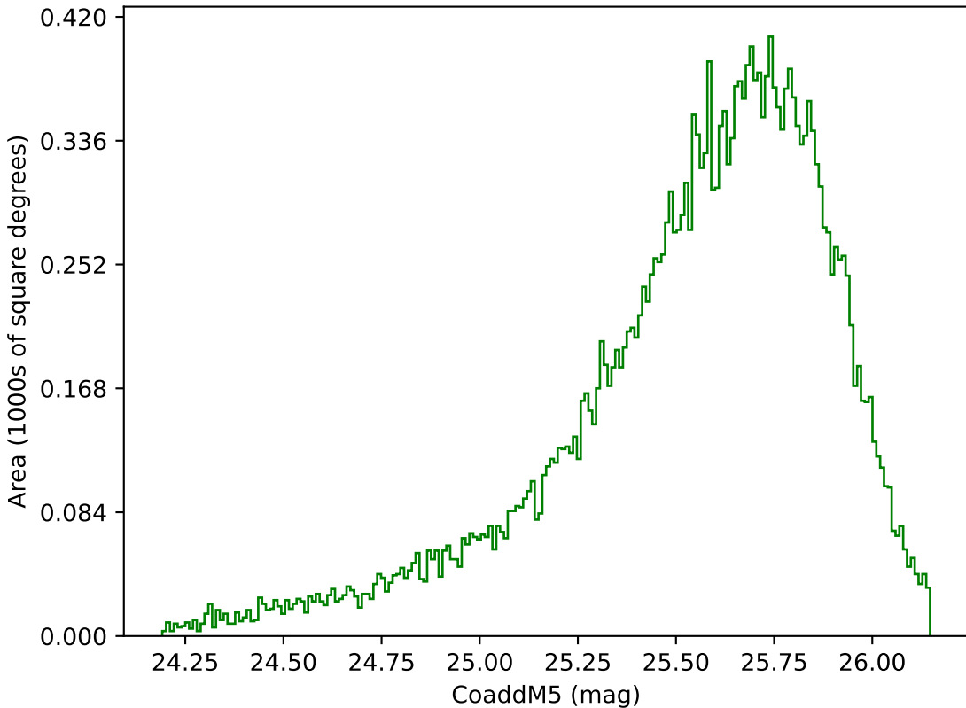
weather_cloudso30v3.4_10yrs Yr 1 g band: CoaddM5
