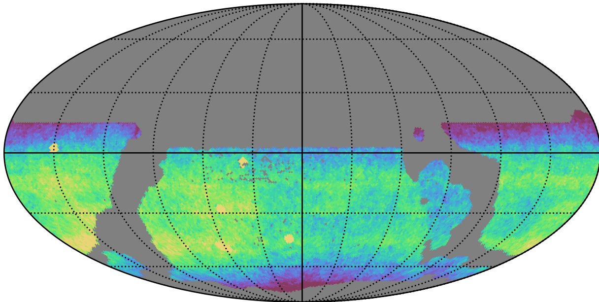
weather_cloudso30v3.4_10yrs WFD z band: CoaddM5
