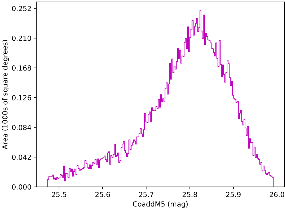
weather_cloudso30v3.4_10yrs WFD z band: CoaddM5
