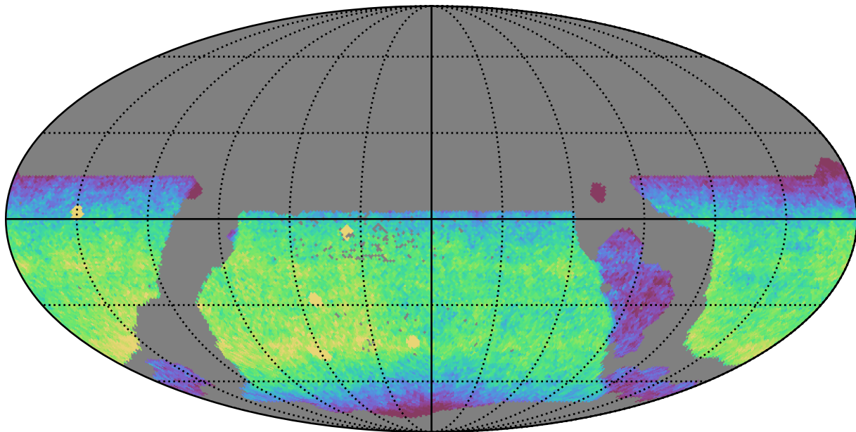
weather_cloudso30v3.4_10yrs WFD y band: CoaddM5
