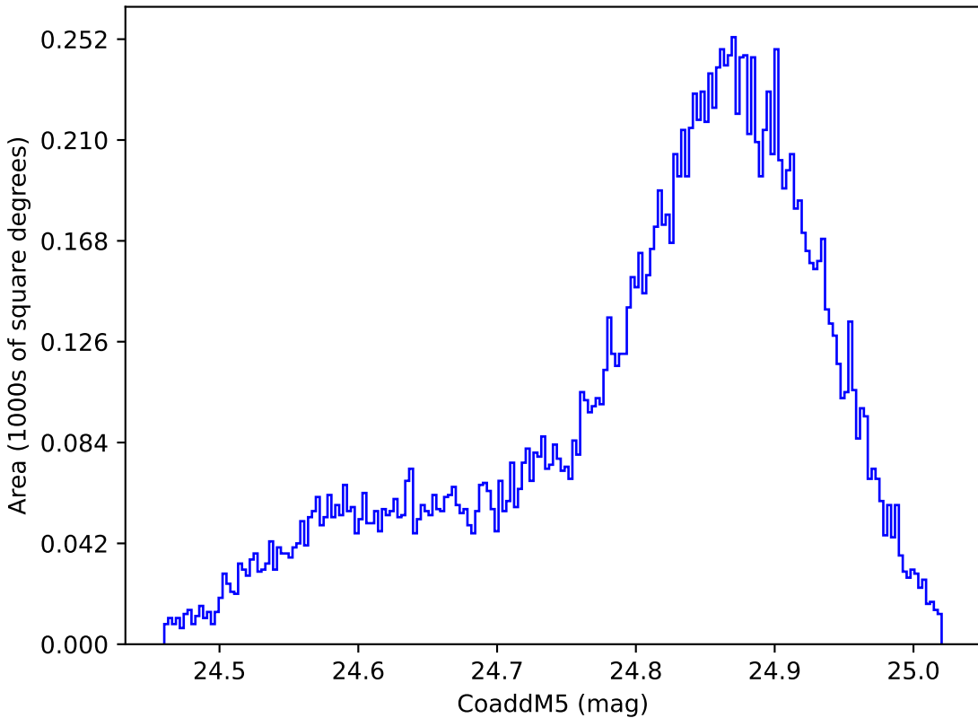
weather_cloudso30v3.4_10yrs WFD y band: CoaddM5
