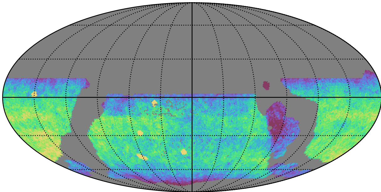
weather_cloudso30v3.4_10yrs WFD u band: CoaddM5
