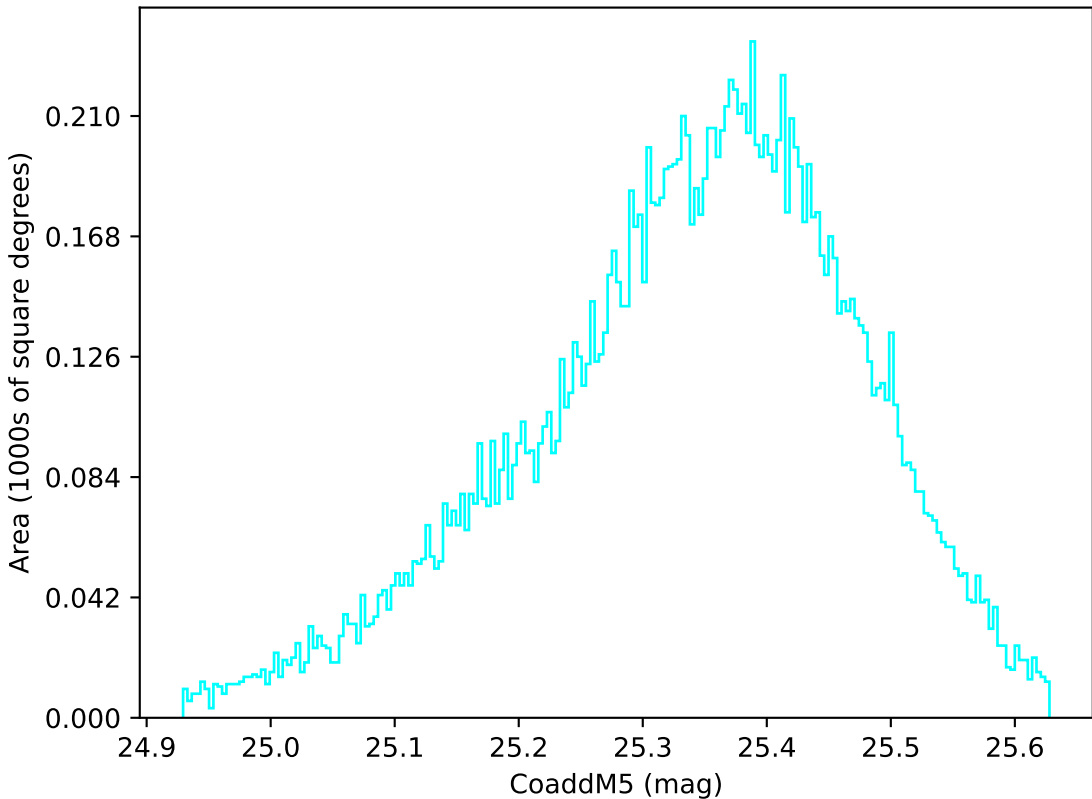
weather_cloudso30v3.4_10yrs WFD u band: CoaddM5
