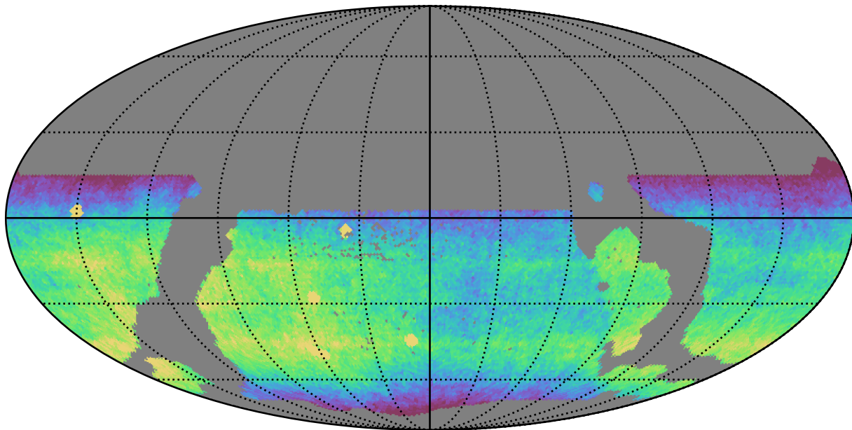
weather_cloudso30v3.4_10yrs WFD r band: CoaddM5
