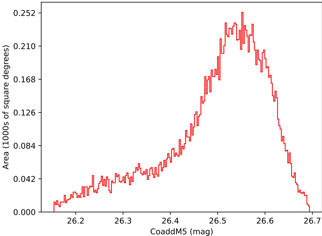
weather_cloudso30v3.4_10yrs WFD i band: CoaddM5
