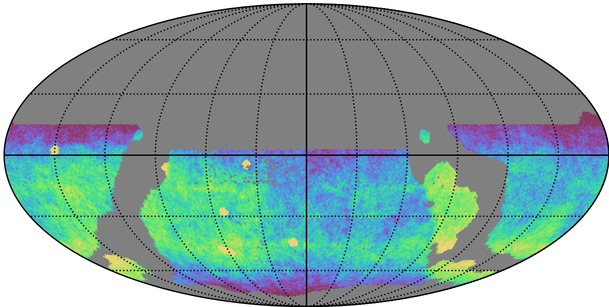
weather_cloudso30v3.4_10yrs WFD g band: CoaddM5
