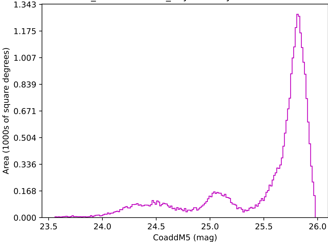
weather_cloudso30v3.4_10yrs All sky z band: CoaddM5
