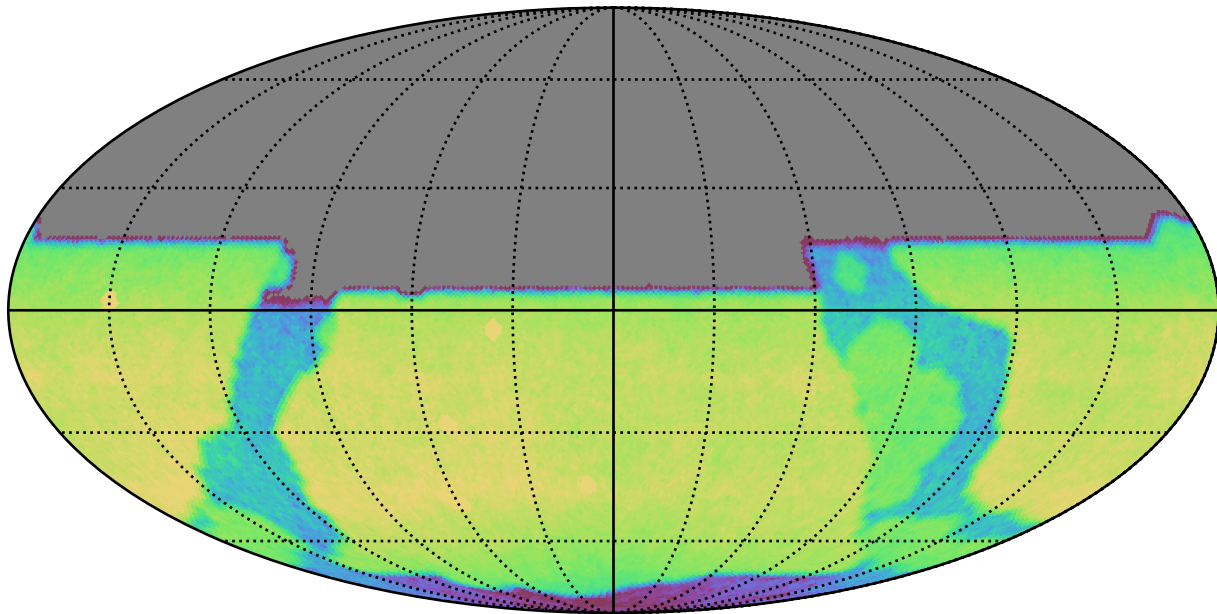
weather_cloudso30v3.4_10yrs All sky y band: CoaddM5
