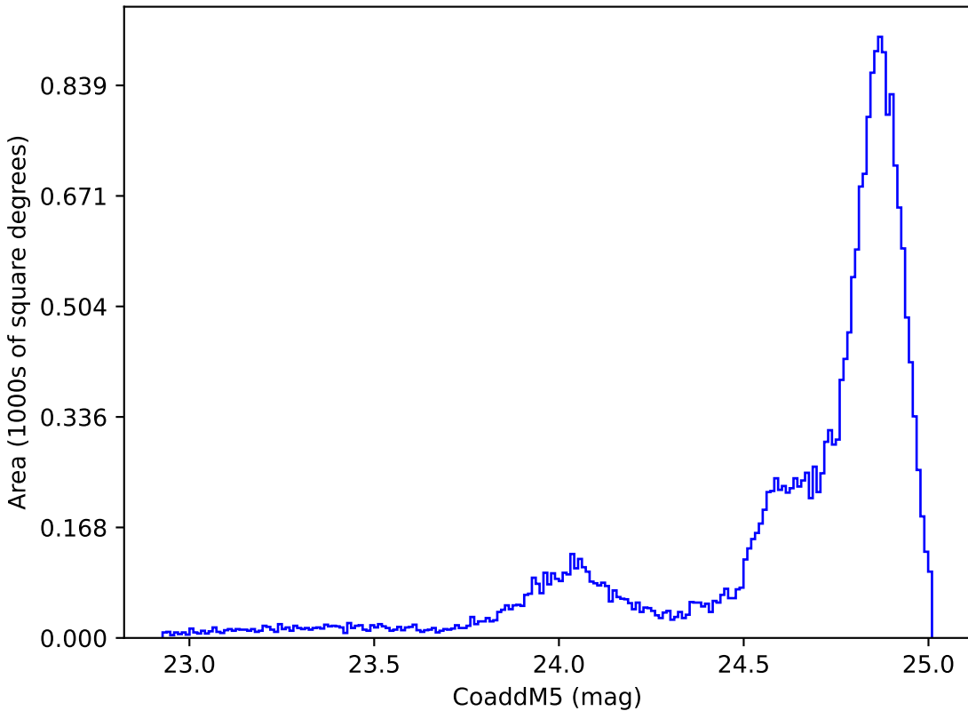
weather_cloudso30v3.4_10yrs All sky y band: CoaddM5
