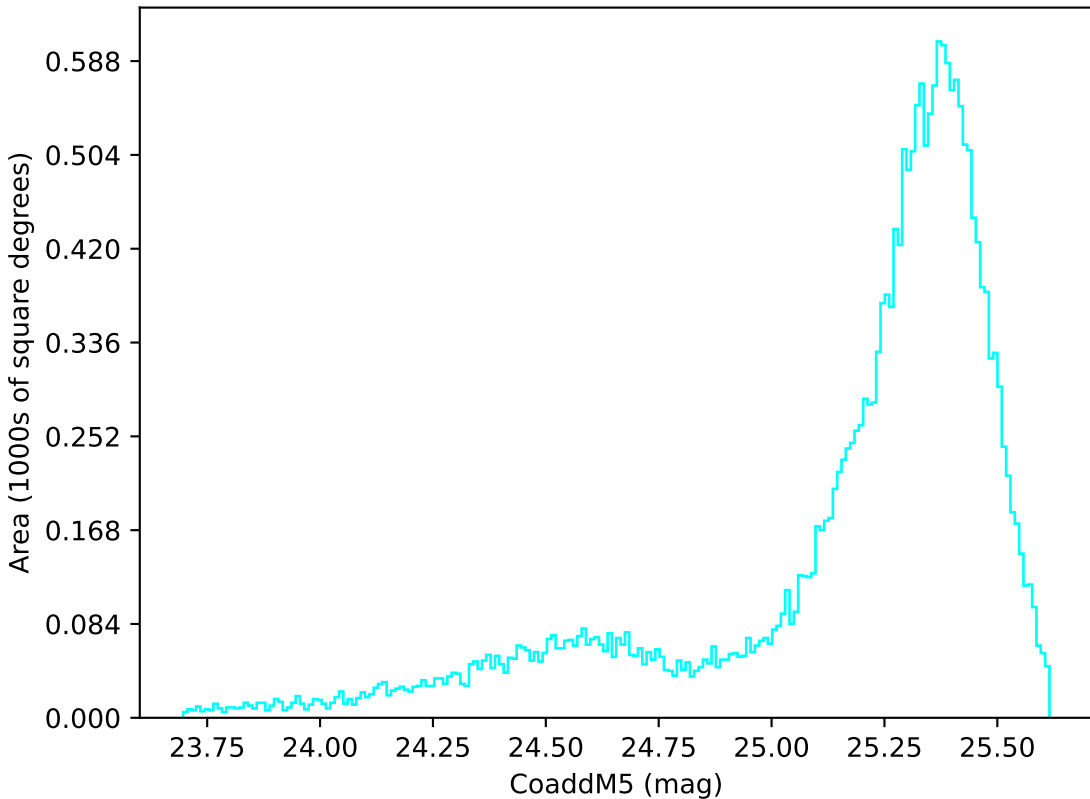
weather_cloudso30v3.4_10yrs All sky u band: CoaddM5
