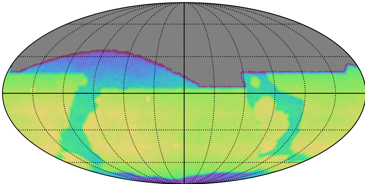
weather_cloudso30v3.4_10yrs All sky r band: CoaddM5
