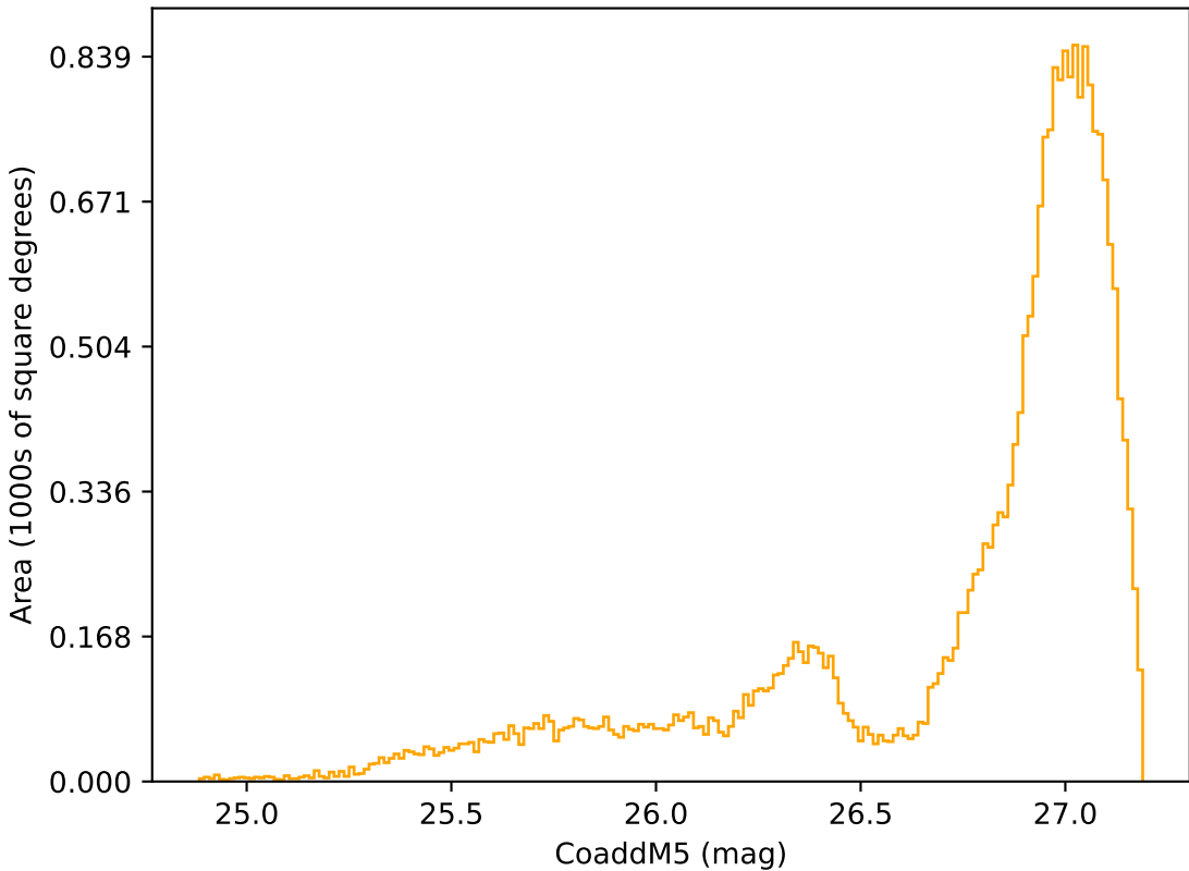
weather_cloudso30v3.4_10yrs All sky r band: CoaddM5
