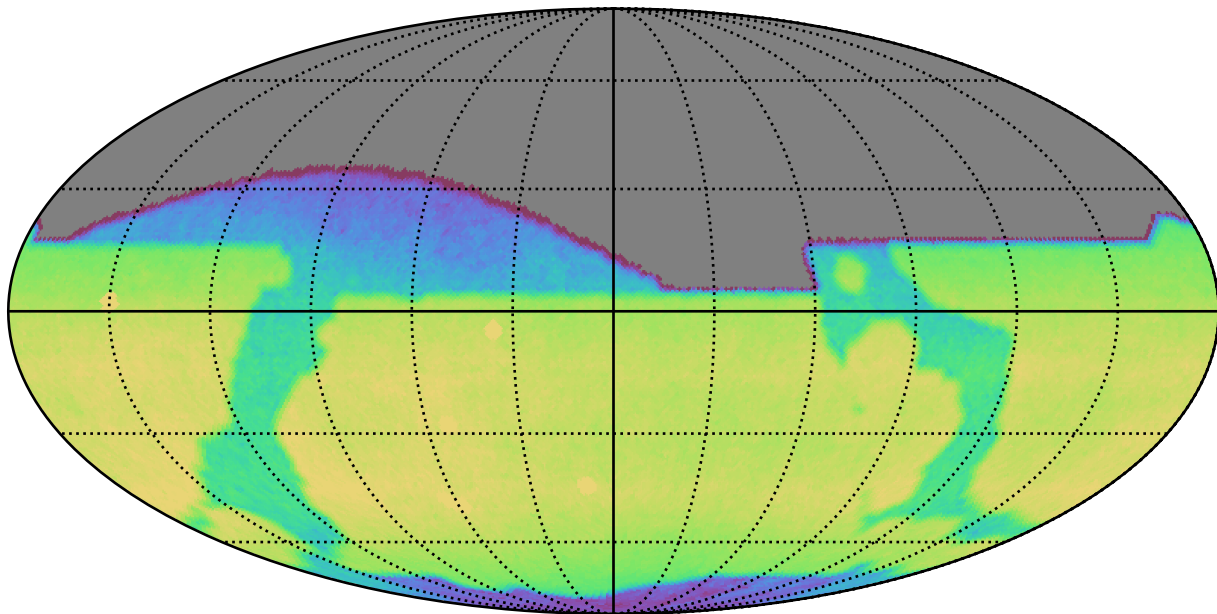
weather_cloudso30v3.4_10yrs All sky i band: CoaddM5
