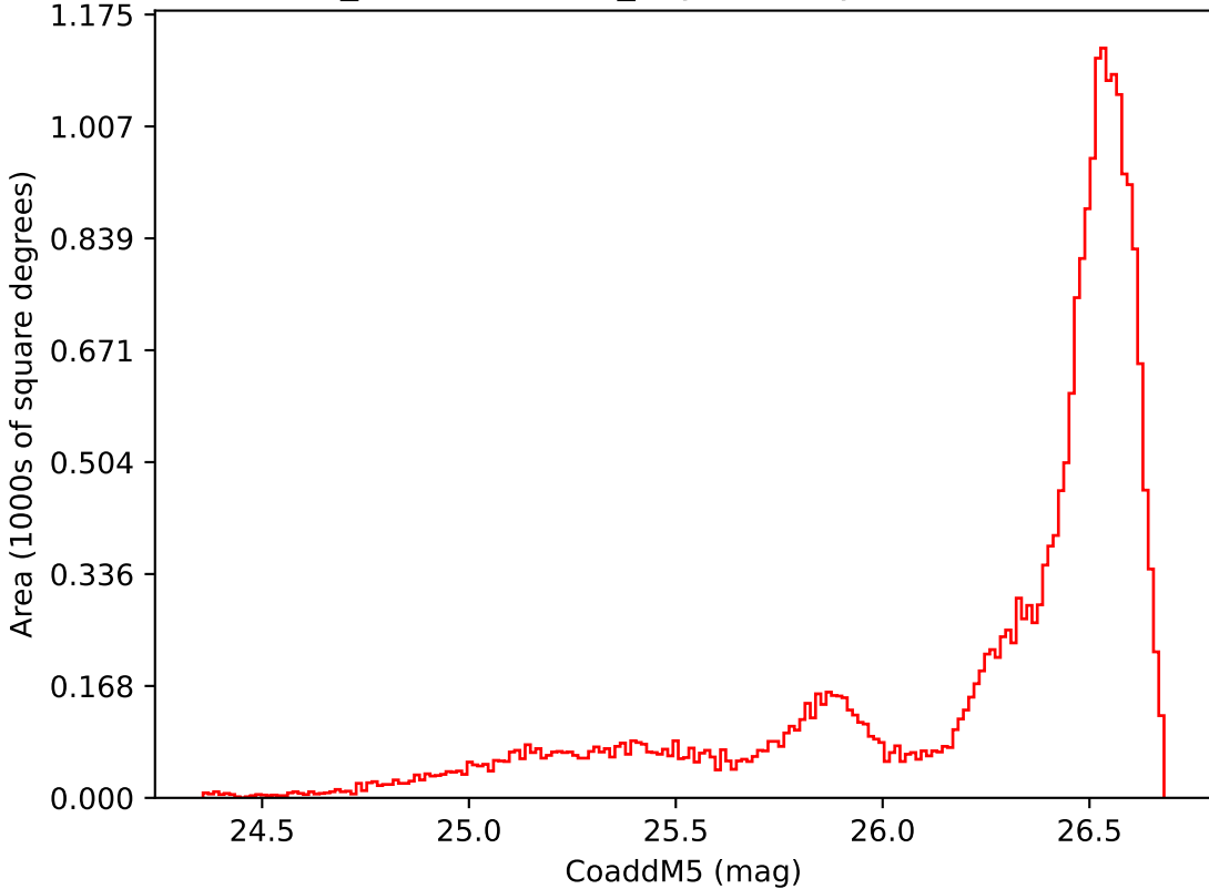
weather_cloudso30v3.4_10yrs All sky i band: CoaddM5
