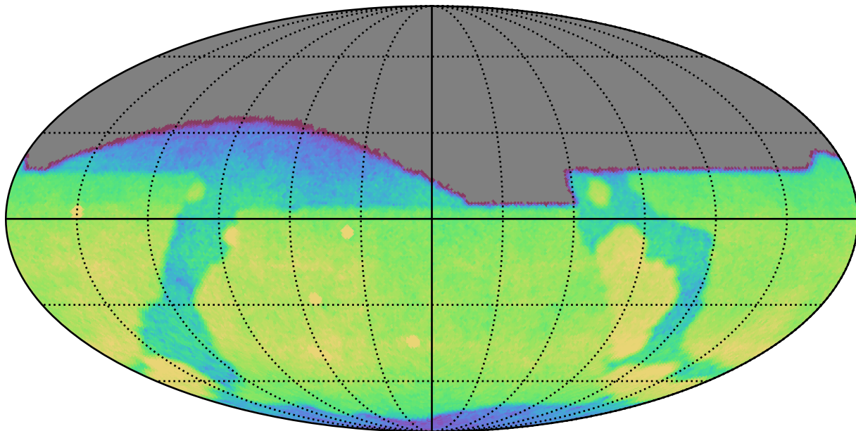
weather_cloudso30v3.4_10yrs All sky g band: CoaddM5
