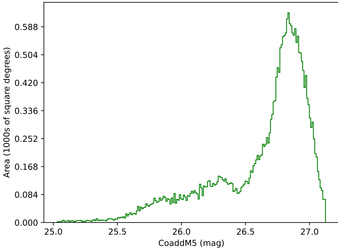
weather_cloudso30v3.4_10yrs All sky g band: CoaddM5
